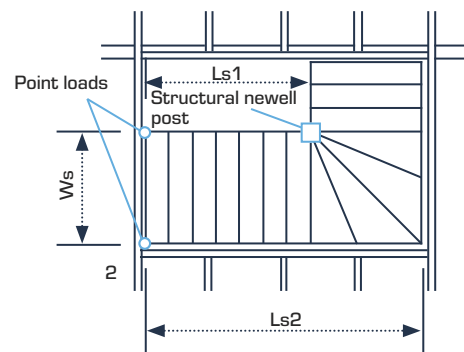
Figure 3.2 Definition of stair width and length for non-straight flights of stairs.
